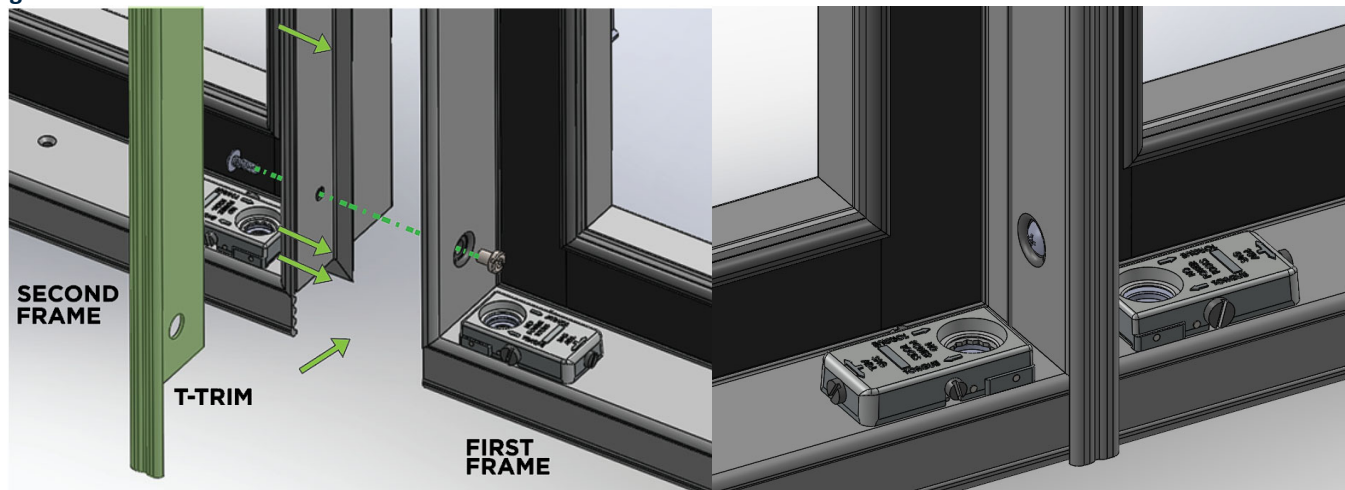
Figure 2.6: T-Trim installation
