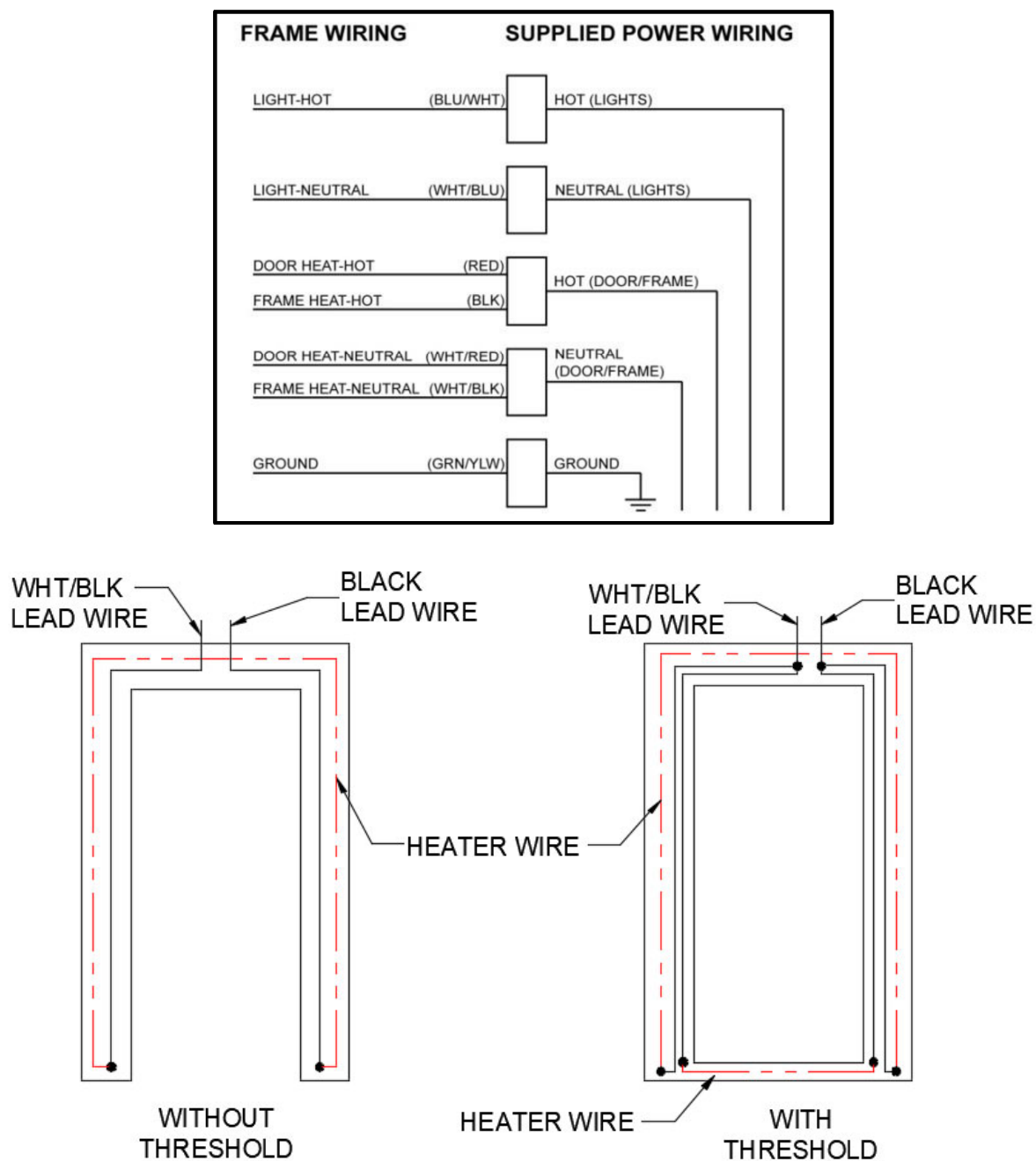
Figure 16.8: Wiring Diagram
