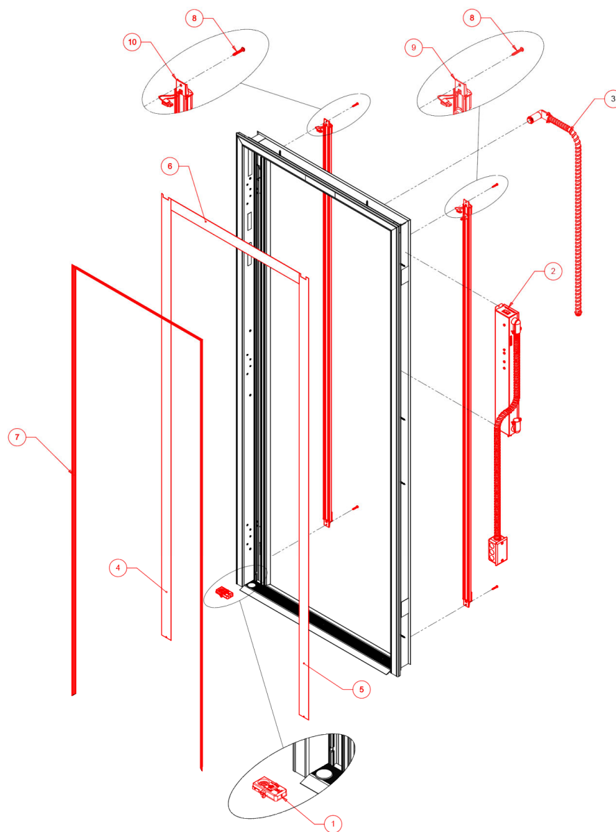
Figure 18.1 Frame Assembly for 403N Series NT Pass-Thru; Replacement Parts
