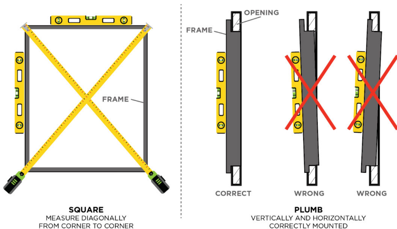
Figure 16.1: Frame Alignment, Squareness, and Plumb
