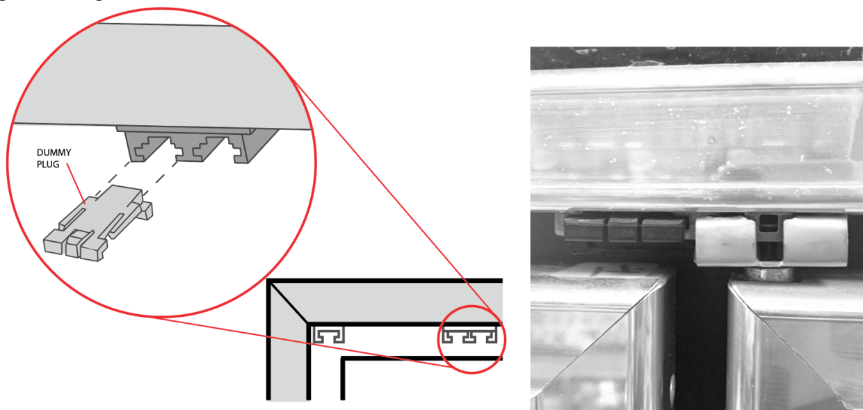
Figure C.2: Plug Removal
