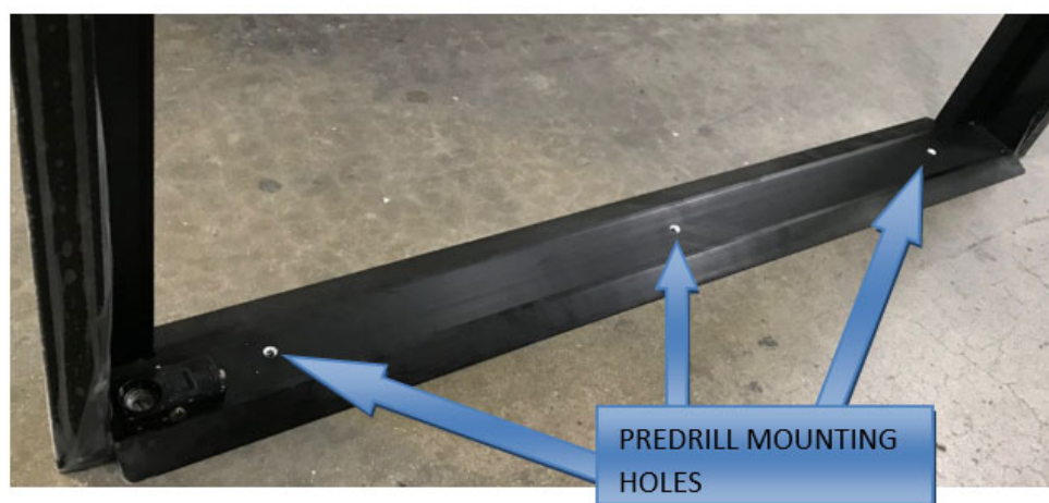
Figure 16.4: Mounting Holes
