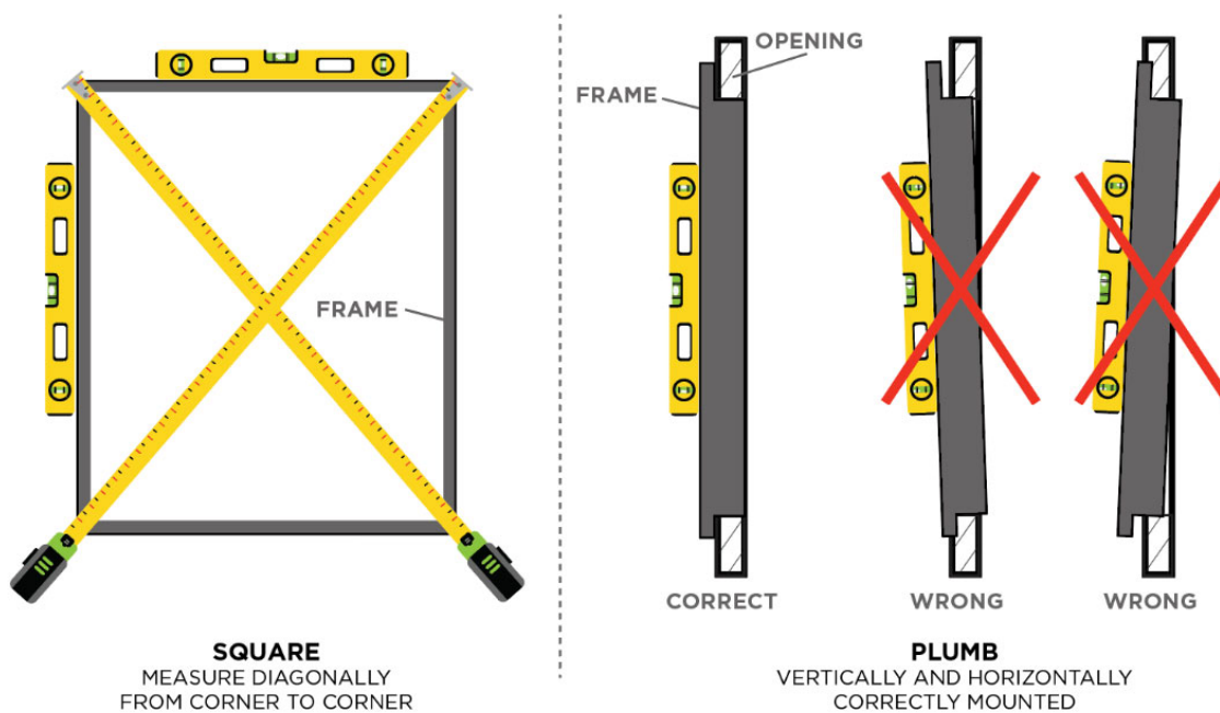
Figure 2.4: Frame Alignment, Squareness, and Plumb
