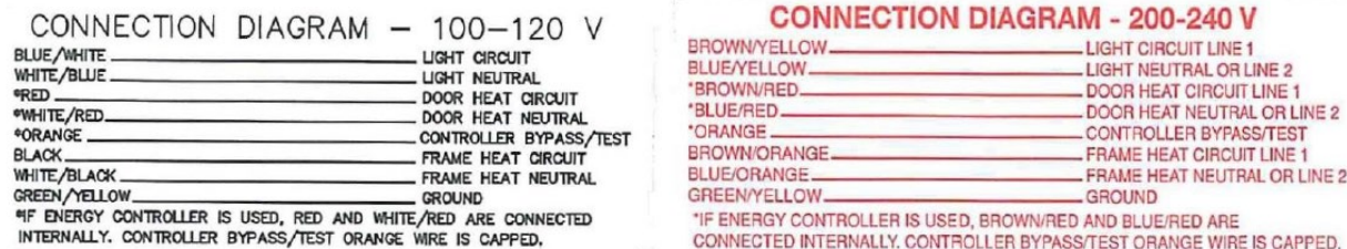
Figure 2.11: Wiring Labels
