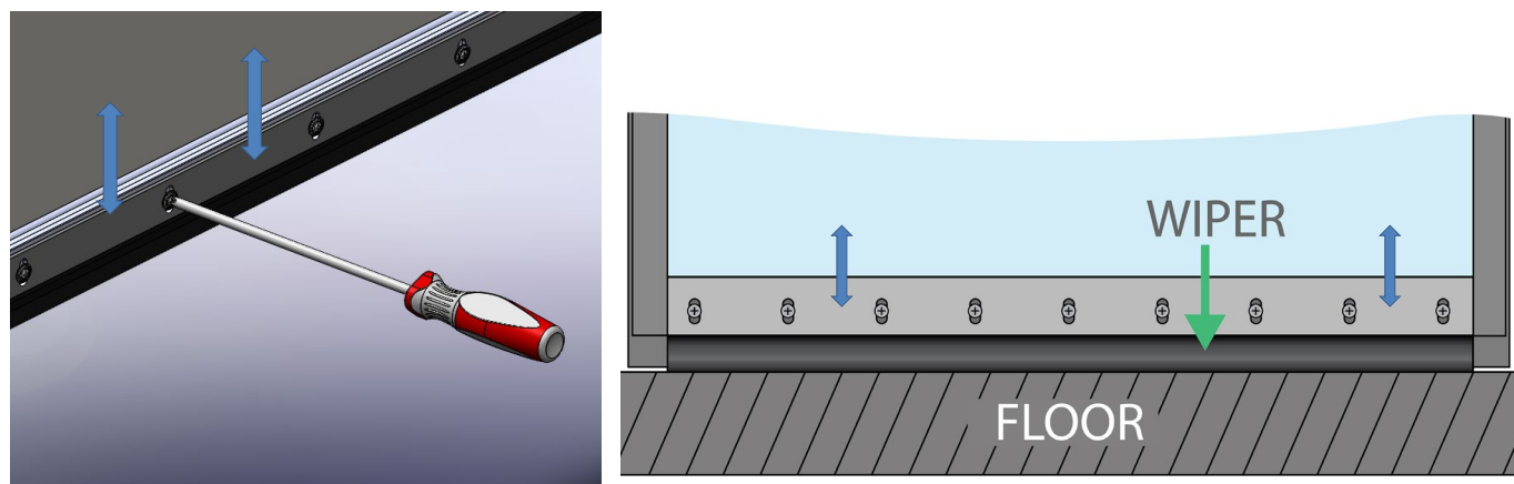
Figure I.1 – Wiper Adjustment
