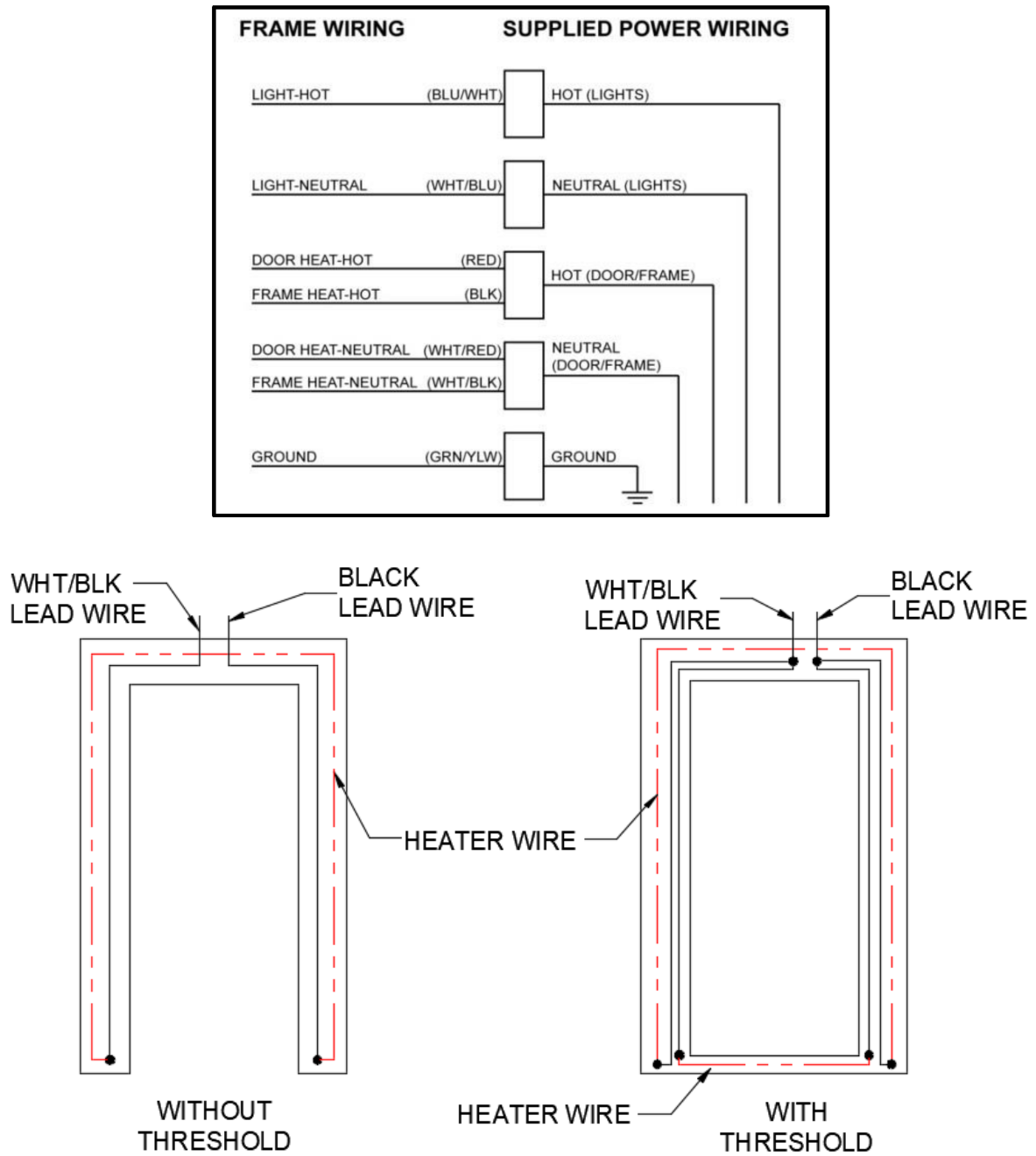
Figure 17.8: Wiring Diagram
