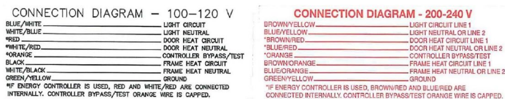
Figure 17.7: Wiring Labels
