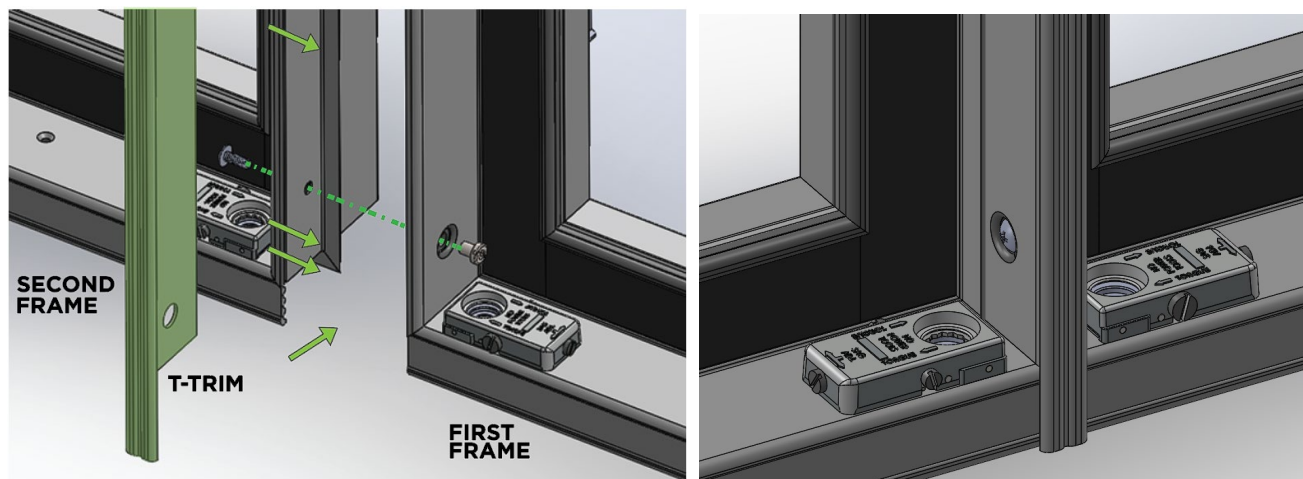
Figure 2.7: T-Trim installation
