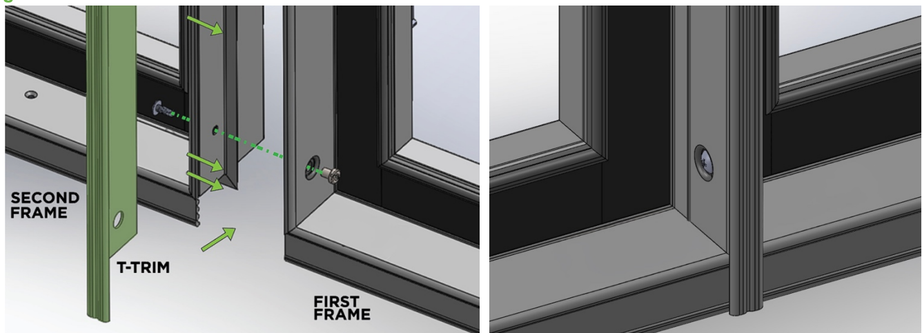
Figure 2.8: T-Trim installation
