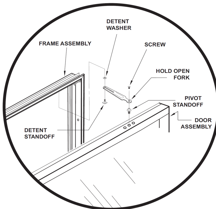
Figure 13.2 Hold-open Assembly
