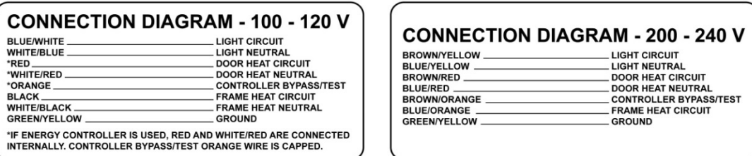
Wire Diagram Connection Label
