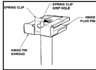
Hinge Pin Assembly
