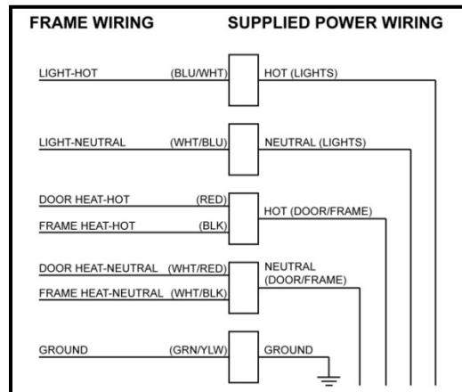
Wiring Diagram
