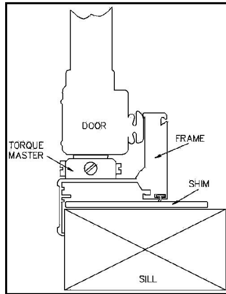
Anthony Door and Frame Cross-Section
